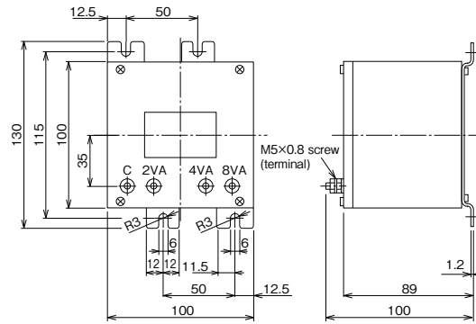
Various characteristics of AN/CN Series current transformers for cubicle type high-voltage power receiving equipment
