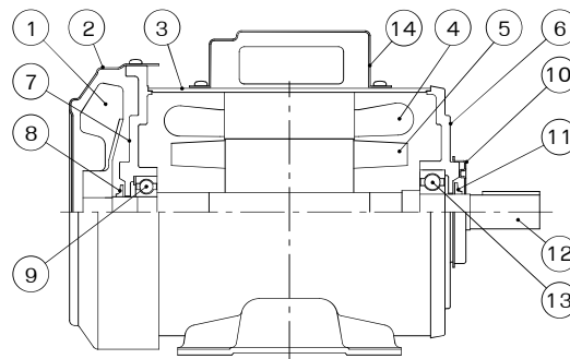
Figure 6: Motor parts
