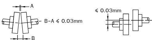
Figure 2: Coupling alignment
