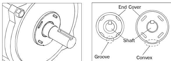
Wearing Type End Cover
