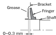
Figure 9: Fringer re-assembly & alignment
