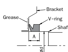
Figure 10: V-ring re-assembly
